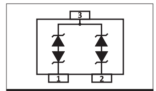
PIN CONFIGURATIONS
